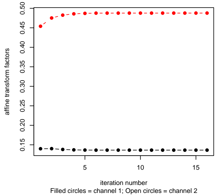
6d. Convergence of vsn robust fit
