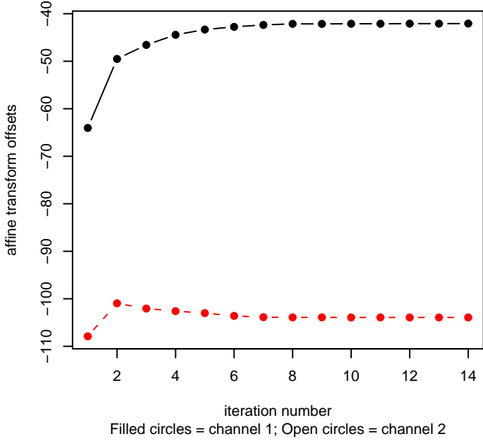
6c. Convergence of vsn robust fit
