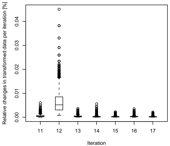
6d. Convergence of vsn robust fit
