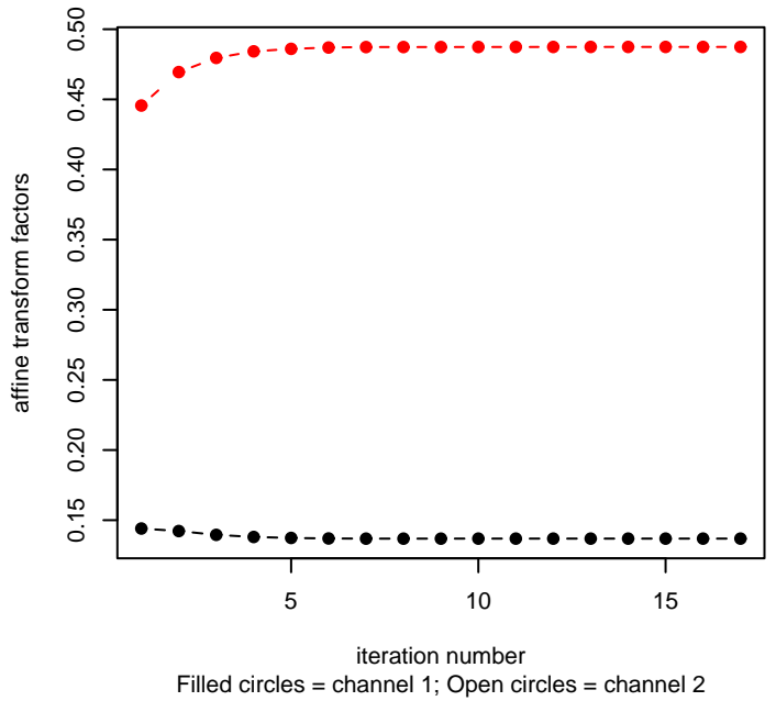
6b. Convergence of vsn robust fit
