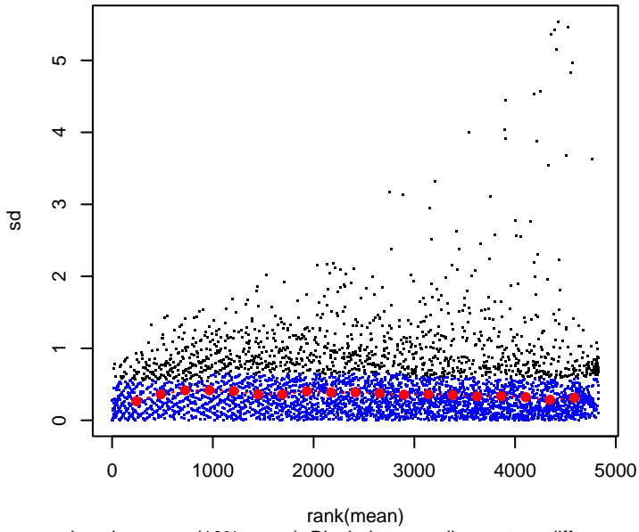
5a. Data after variance stabilizing normalization (vsn)
