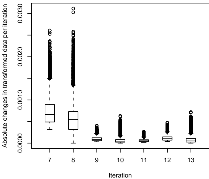
6c. Convergence of vsn robust fit
