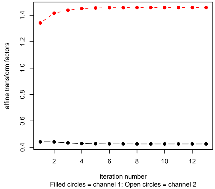
6d. Convergence of vsn robust fit
