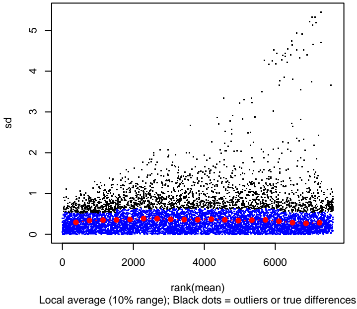
6a. Convergence of vsn robust fit
