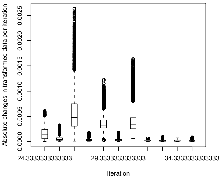
6c. Convergence of vsn robust fit
