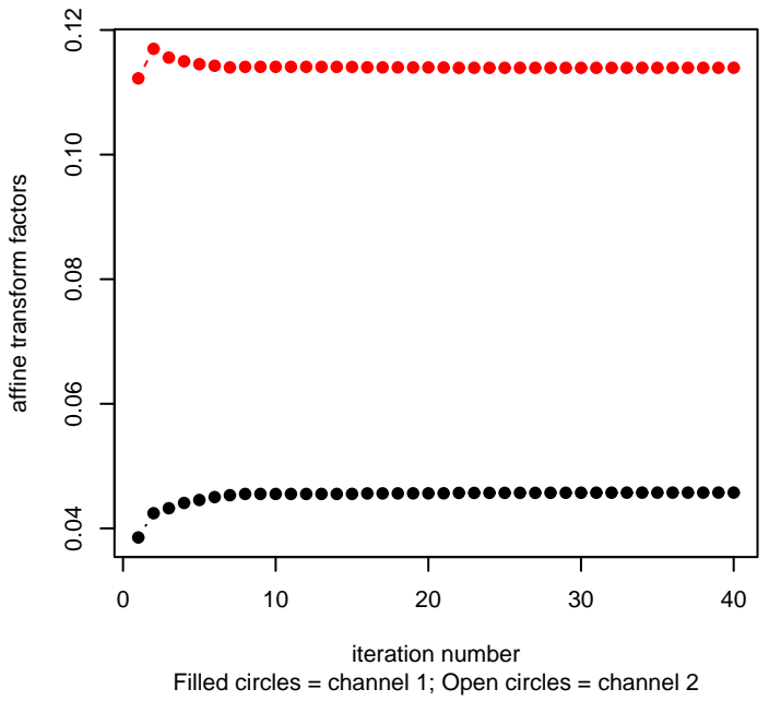
6b. Convergence of vsn robust fit
