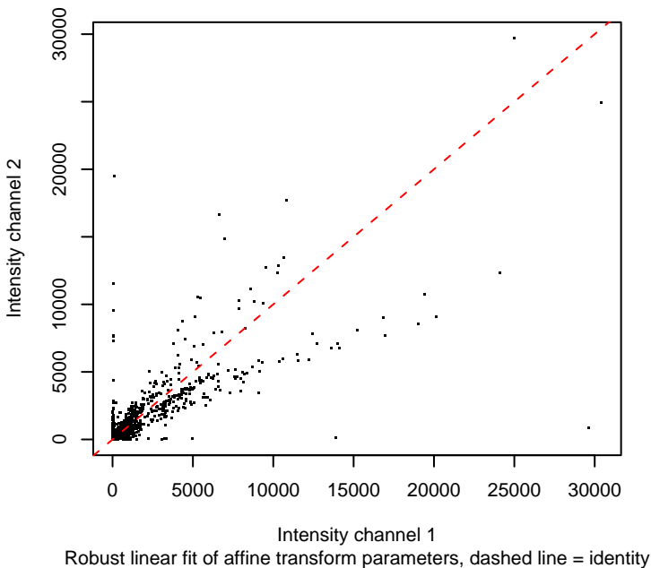
4. Data after variance stabilizing normalization (vsn)
