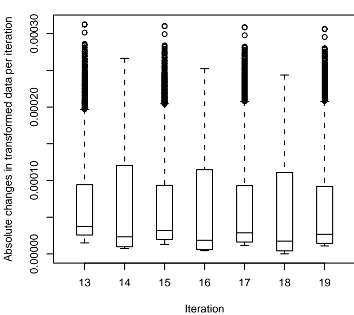
6c. Convergence of vsn robust fit
