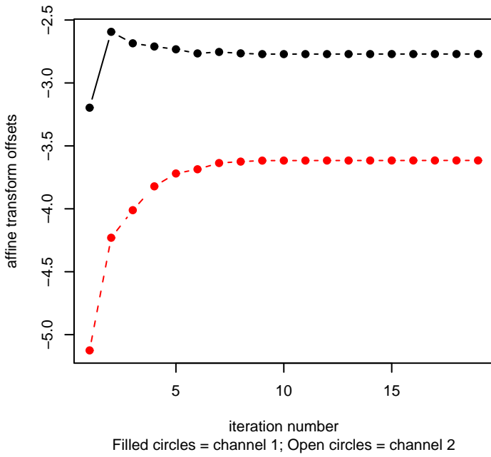
6a. Convergence of vsn robust fit
