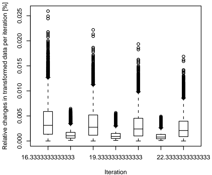
6d. Convergence of vsn robust fit
