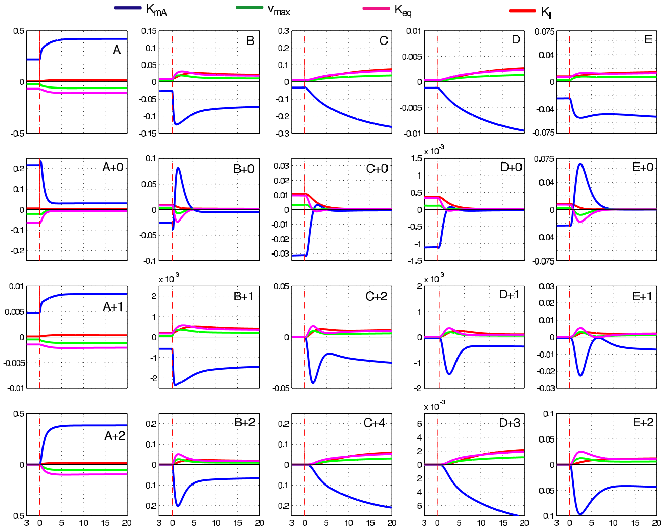
Figure 7 Parameter sensitivity plots. First row: Sensitivities of the concentrations to the parameters of reaction v_1 ( K_{mA} , v_{max} and K_{eq} ) and v_{upt} ( K_i ). Second to last row: Sensitivities of selected mass isotopomer concentrations to the same parameters.
